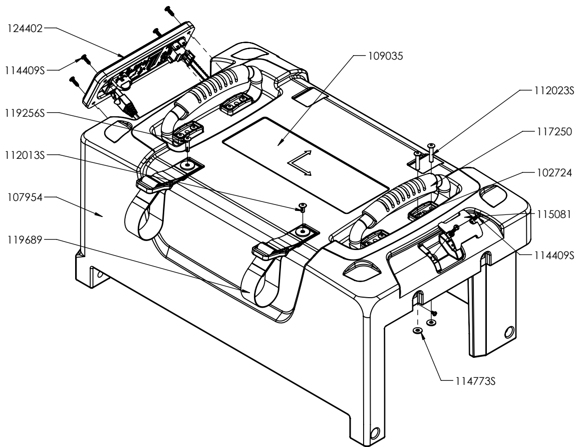
TOP ASSEMBLY
