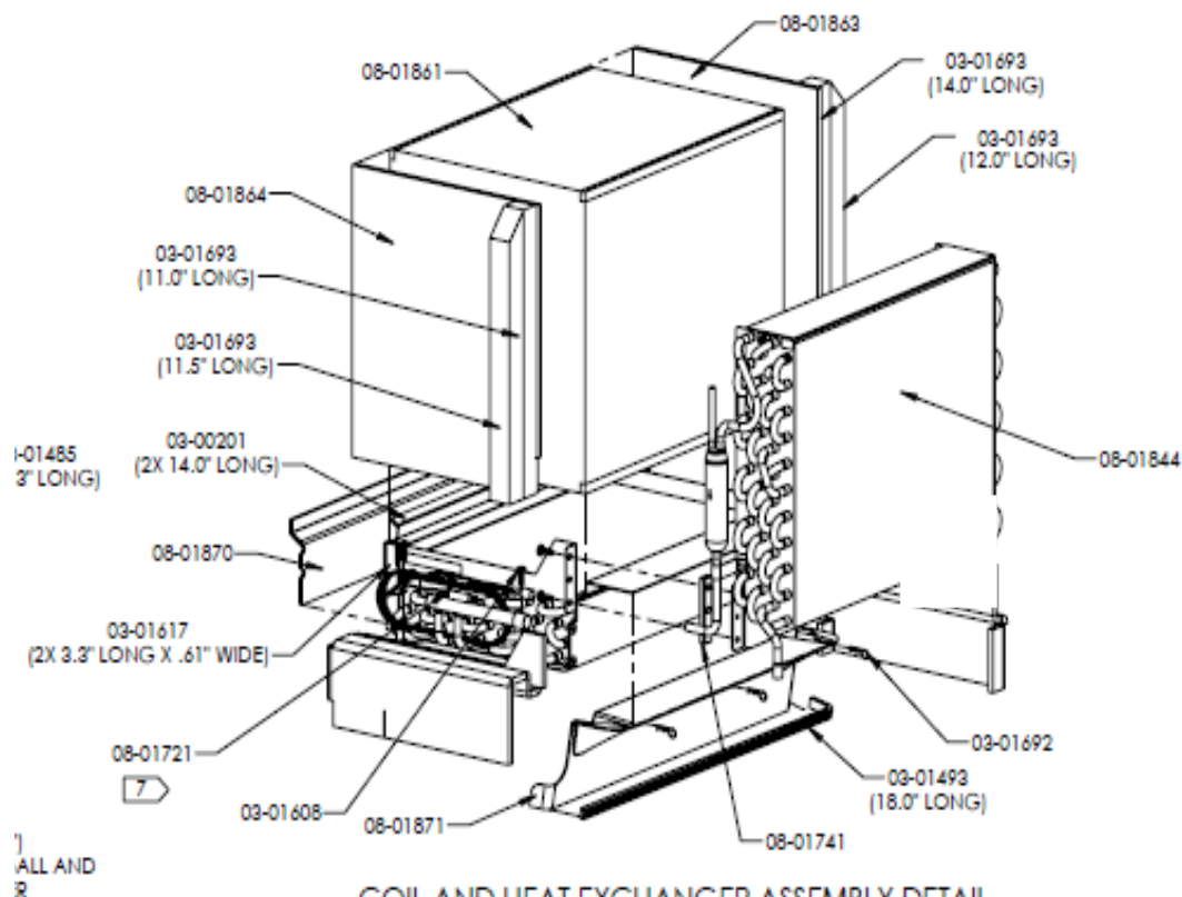
COIL AND HEAT EXCHANGER ASSEMBLY DETAIL
