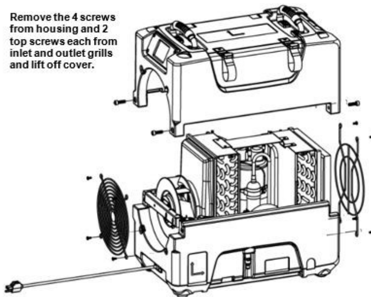
Fig. B: Disassembly for Cleaning
