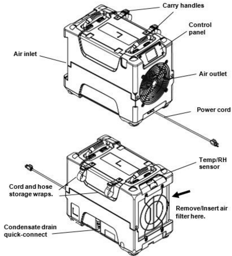
Fig. A: Parts Identification
